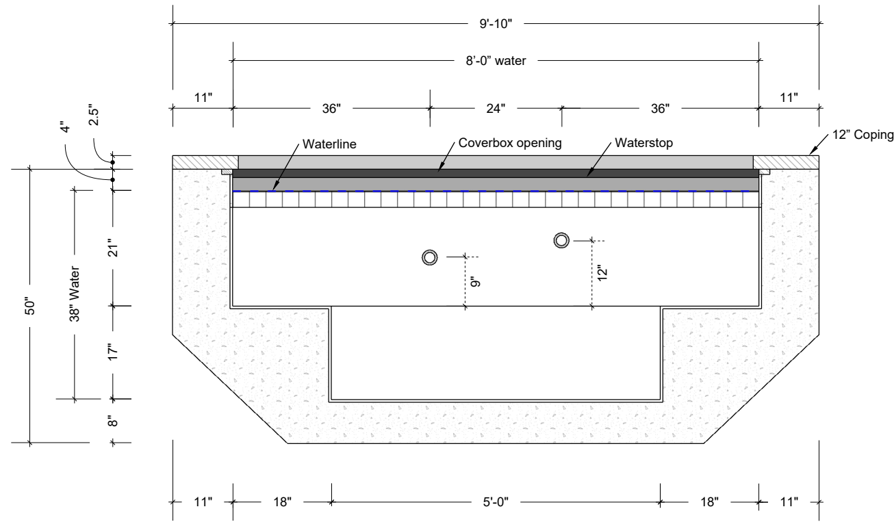
2 Spa Elevation PL6 Scale: 1/2" = 1FT Follow Measures
