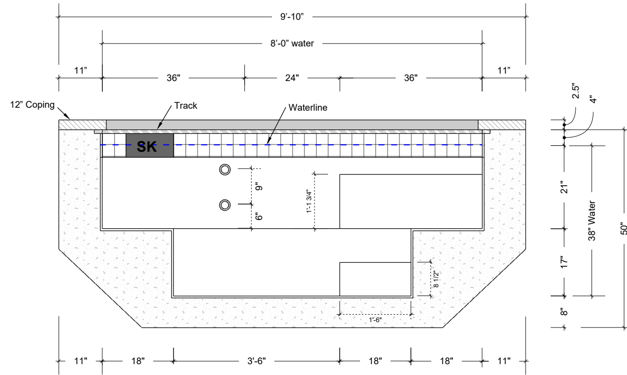
1 Spa Elevation PL6 Scale: 1/2" = 1FT Follow Measures
